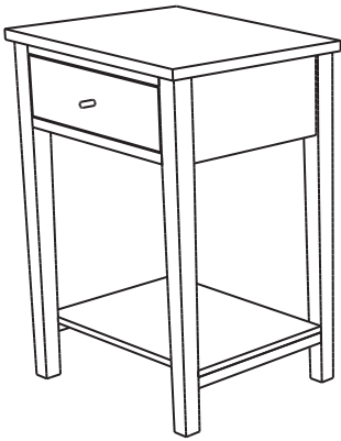
Bedside table drawer & shelf 420W 370D 640H Feature Ash $935 Jarrah $1045 Red gum $1100 Blackwood $1100
